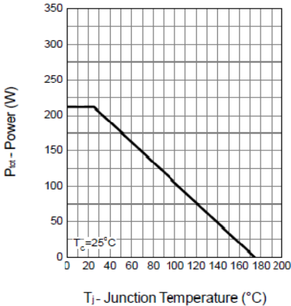
Power Dissipation
